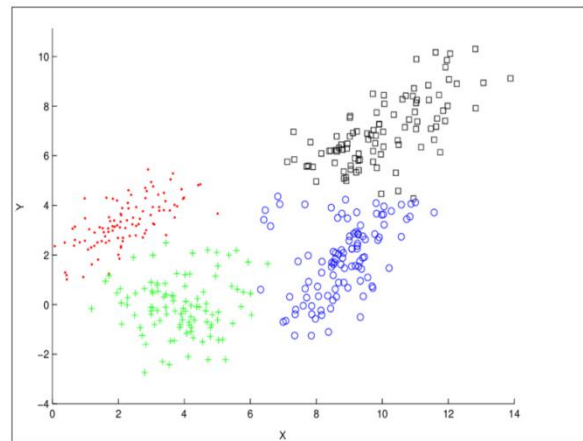
Figure 2 clustering example
