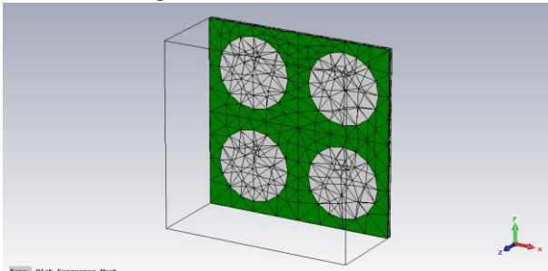
Fig .6 Mesh details of the Frequency-Domain Solver in CST MWS
