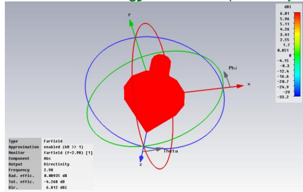
Fig. 4. The far field at frequency F=980MHz
