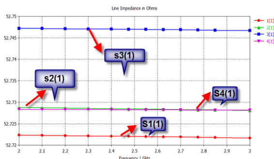
Fig.9 S - impedance of RFID antenna
