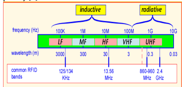
Fig 5.2: RFID frequency Bands [3]
