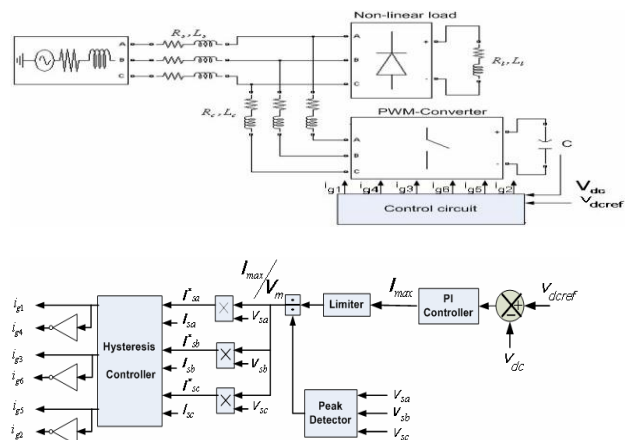
Figure 2 a) Active filter system b) Active filter system using PI controller
