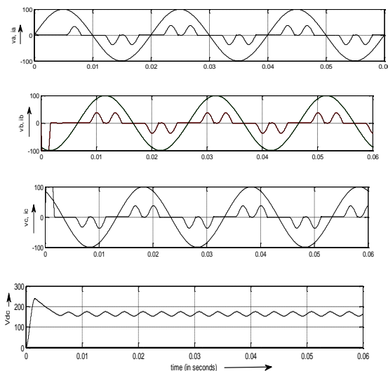
Figure 8 Waveform without controller
