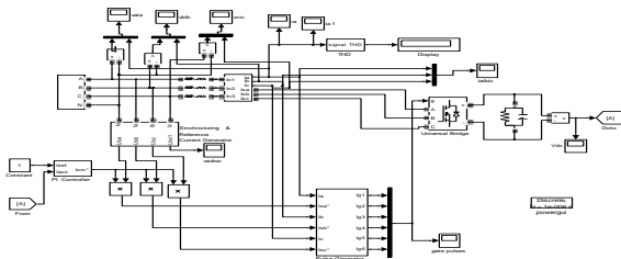
Figure 6 Simulated power circuit for PI controlled improved power quality converter
