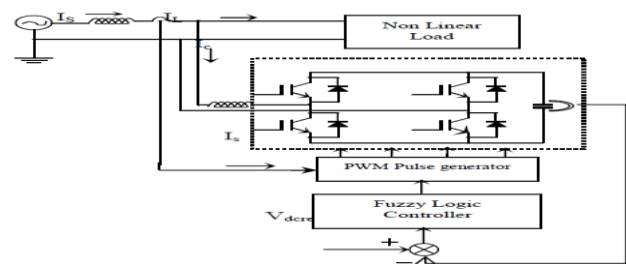
Figure 4 Block Diagram of Fuzzy controlled improved power quality converter
