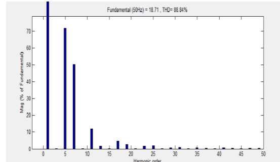
Figure 9 Harmonics spectrum without controller
