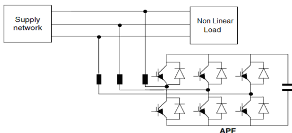
Figure 1 Active power filter connected with transmission line
