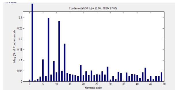
Figure 10 Harmonics spectrum with PI controller
